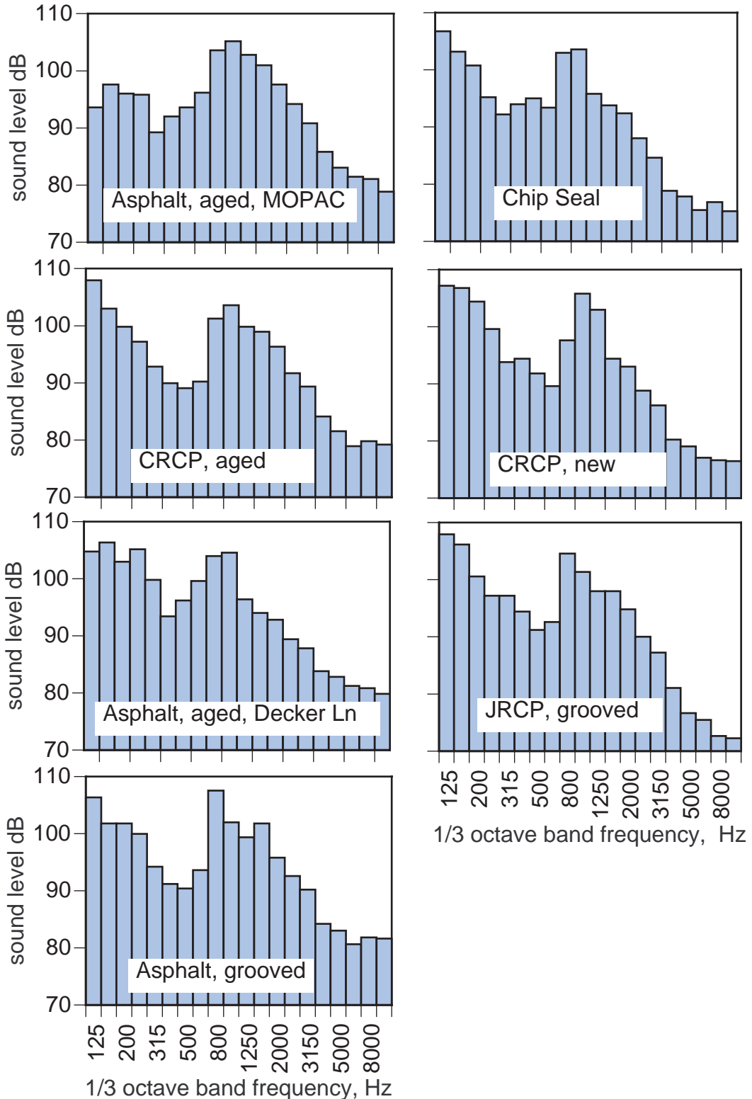
FIGURE 9 (continued). Spectral sound level of 180 degree angle microphone, on board noise of Texas pavements.
