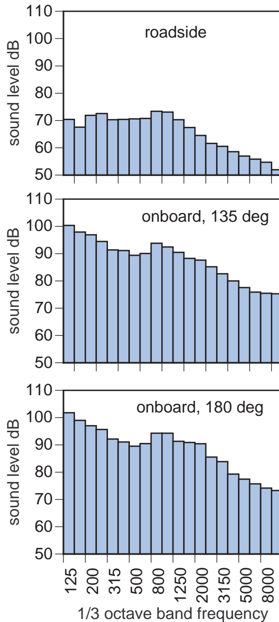
FIGURE 10. Frequency spectrum for aged Novachip recorded at roadside and two onboard, near tire locations. Angle measured from direction of travel.
