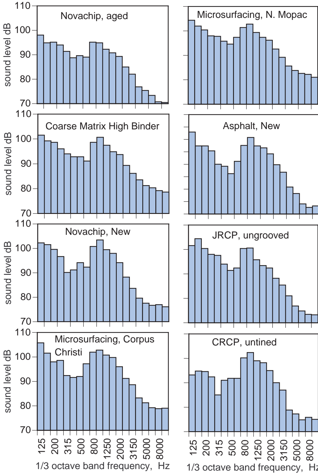
FIGURE 9. Spectral sound level of 180 degree angle microphone, on board noise of Texas pavements.
