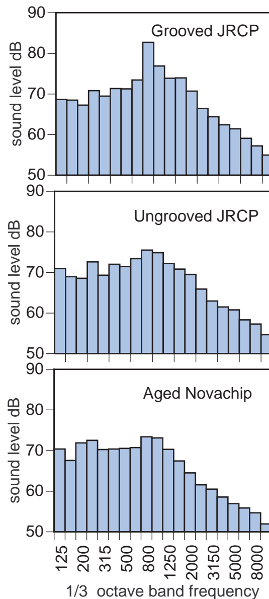
FIGURE 7. Frequency spectrum of three different pavements for comparison.
