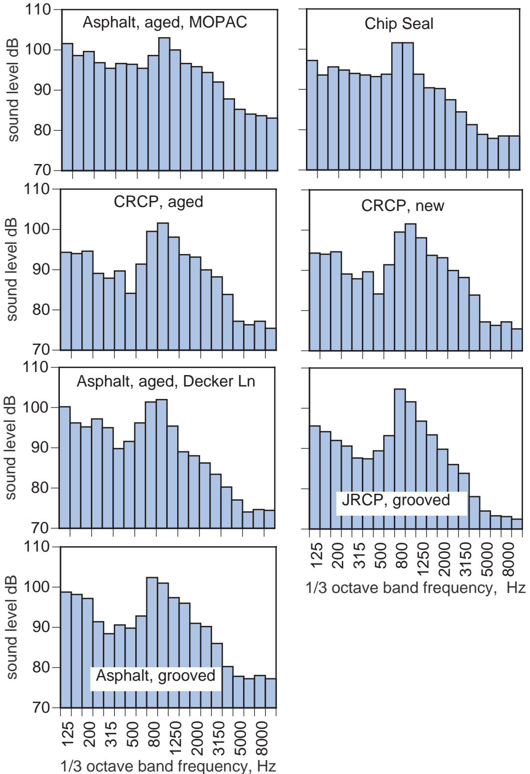
FIGURE 8 (continued). Spectral sound level of 135 degree angle microphone, on board noise of Texas pavements.
