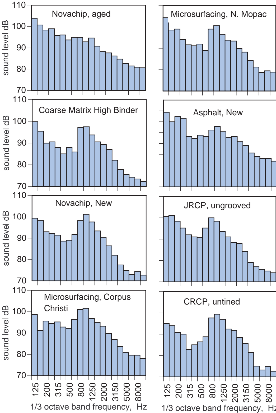
FIGURE 8. Spectral sound level of 135 degree angle microphone, on board noise of Texas pavements.
