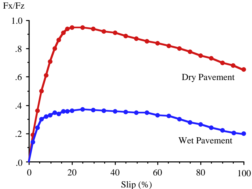
Figure 2. Longitudinal force versus slip.
