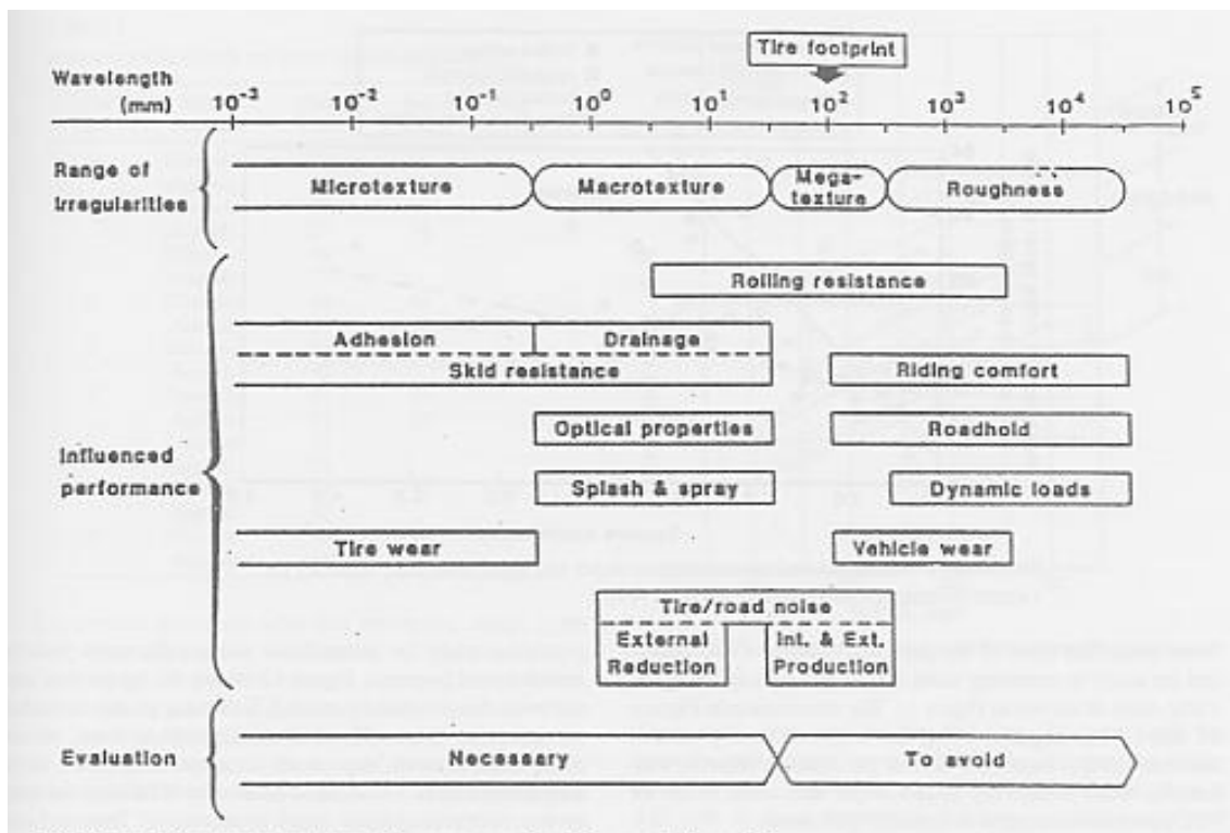
Figure 1. Influence of surface characteristics on vehicle performance.
