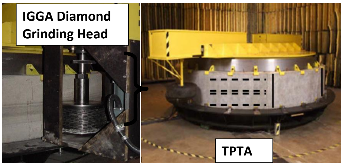
Figure 1- Purdue Tire Pavement Test Apparatus and IGGA Diamond Grinding Head 2
