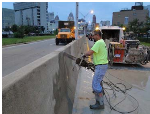
Figure 32. Saw cutting concrete barrier wall to relieve pressure
