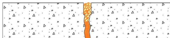
Figure 10. Coarse particles infiltrate joint and expansion occurs
